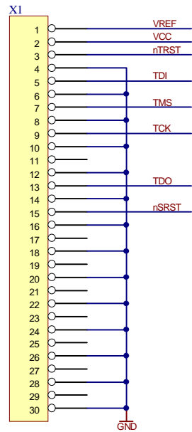
MOLEX FFC-Connector 30pol 0524353072
